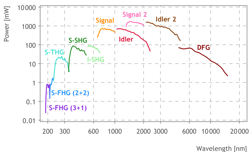
Typical Tuning Curve
